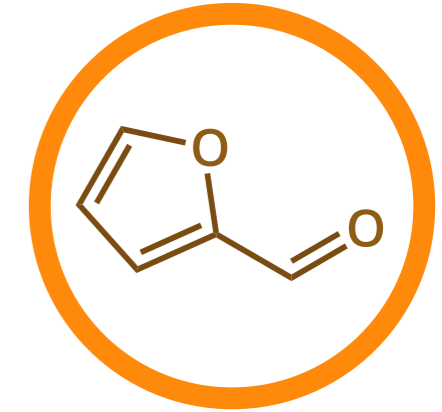
FURFURAL
