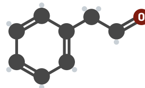
Phenylacetaldehyde
