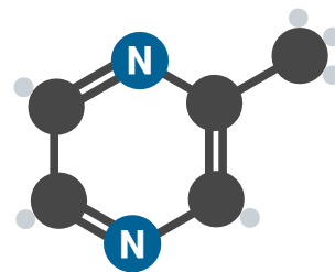
2-methylpyrazine
