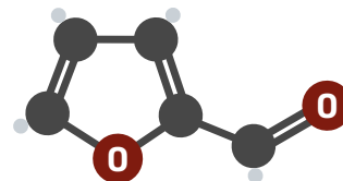
Furfural
